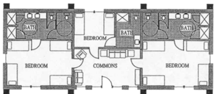
PROPOSED FLOOR PLAN
